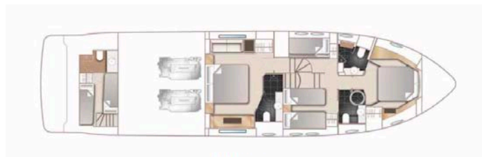
LOWER DECK
